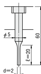
[Fig.4] Buckling of punch
