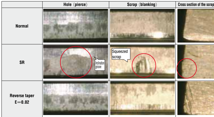
[Fig.8] Cut out section textures for different die shapes
