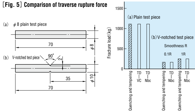
[Fig. 5] Comparison of traverse rupture force
