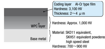
[Fig 1] Cross-sectional view of the RW coating structural model
