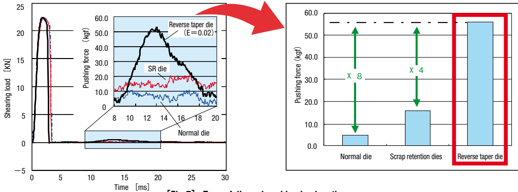
[Fig.7] Type of die and pushing load on the scrap
