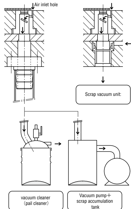
[Fig. 2] Examples of combinations with different vacuum devices
