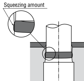
[Fig.5] As the punch goes on penetrating the inner diameter of the reverse taper die goes on decreasing. Therefore, the frictional force between the scrap and die increases because of the squeezing effect on the scrap. As a result, the scrap lifting is prevented.
