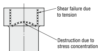
[Fig. 4] Punch head destruction
