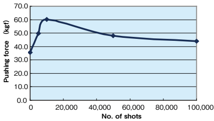
[Fig.9] Comparison of frictional forces for reverse taper dies
