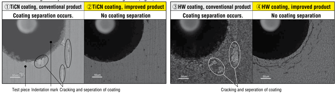
(Fig. 1) Results of observation after indentation test (test piece material: SKH51)
