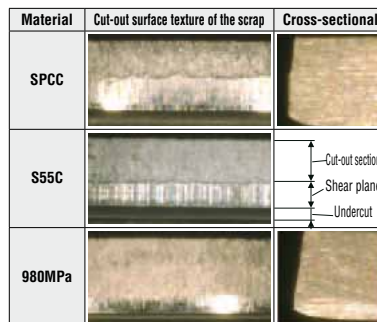
[Fig.2] Cut-out surface texture of the scrap
