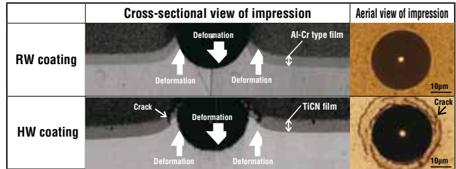
[Fig 1] Evaluation of adhesive capability of the film through Rockwell impression test
