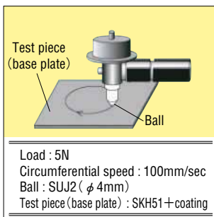
(Fig. 2) Overview of friction wear test
