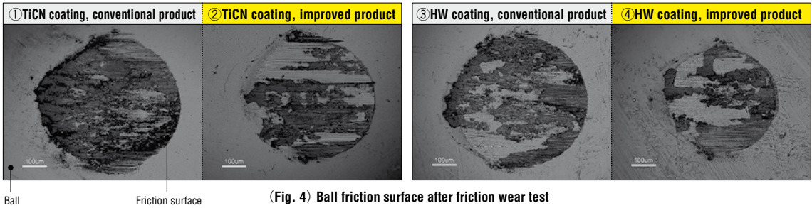
(Fig. 4) Ball friction surface after friction wear test
