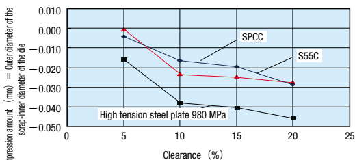
Effect of the materials to be processed on the outer diameter of the scrap [Fig.1] (normal die, \phi 10 , T=1\text{mm} )
