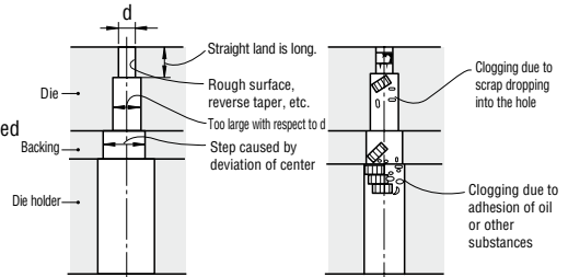
[Fig. 1] Causes of scrap clogging
