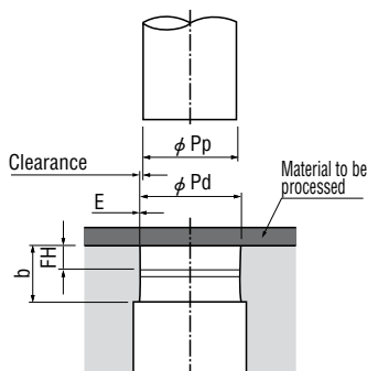
[Fig.3] Before punching
