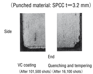
[Fig. 4] Cross-section structure of punch tip after use
