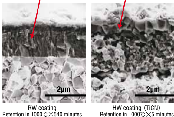
[Fig 2] Heat Test Cross-sectional structure observation
