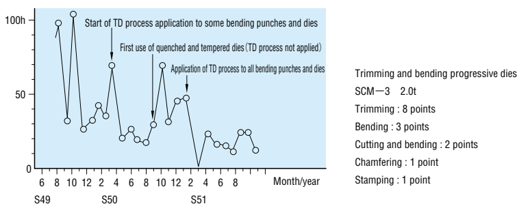
[Fig. 6] Changes in die repair index by TD treatment
