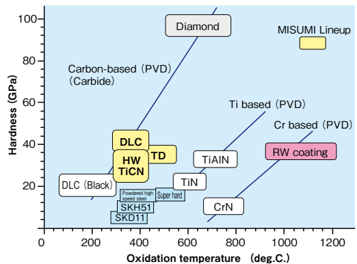
[Fig 3] Relationship between film hardness and heat resistance (Image)
