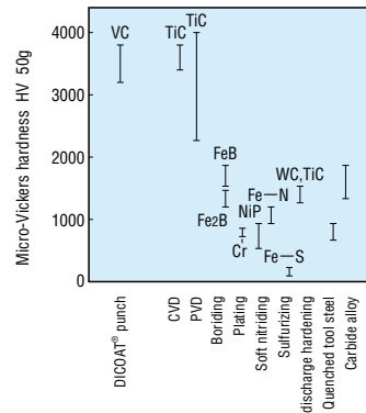
[Fig. 2] Comparison on surface layer hardness
