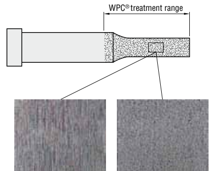
[Fig. 3] Surface comparison of normal polished product and WPC® treated product
