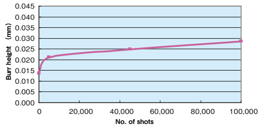
[Fig.10] Change in burr height following the increasing punching count
