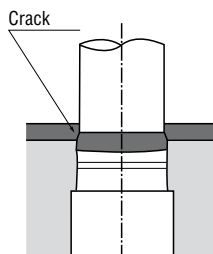
[Fig.4] Cracks in the material to be processed (usual clearance)
